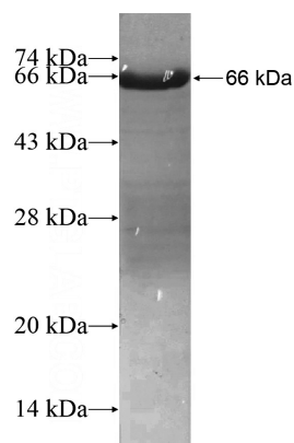
Recombinant Human TDRD3 SDS-PAGE
