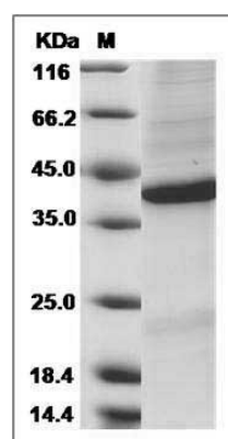
Human FRZB / sFRP-3 Protein (His Tag) SDS-PAGE
