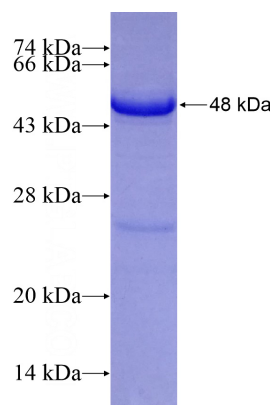
Recombinant Human PLXDC2 SDS-PAGE
