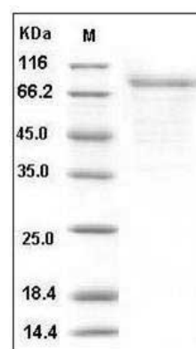
Human CSF2RA / GM-CSFR / CD116 Protein (Fc Tag) SDS-PAGE
