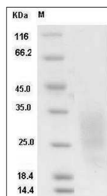
Mouse LAIR1 Protein (His Tag) SDS-PAGE
