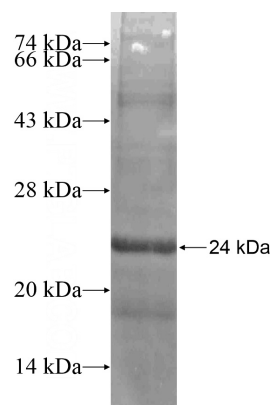
Recombinant Human JUP SDS-PAGE
