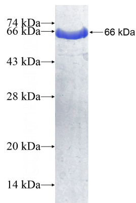
Recombinant Human IFIT3 SDS-PAGE
