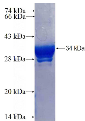
Recombinant Human GNB5 SDS-PAGE
