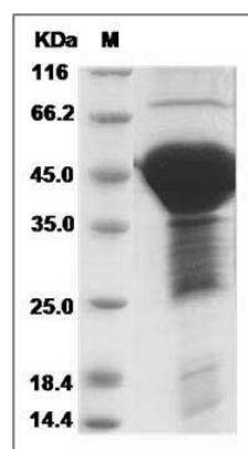
Human MAPT / Tau Protein (His Tag) SDS-PAGE
