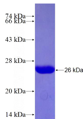
Recombinant Human PEAR1 SDS-PAGE
