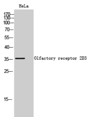
Fig1.: Western Blot analysis of HeLa cells using Olfactory receptor 2D3 Polyclonal Antibody
