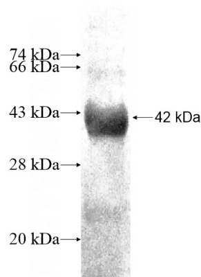
Recombinant Human TDRD7 SDS-PAGE
