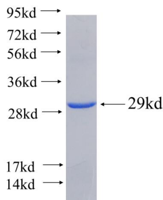
Recombinant human RP11-529I10.4 SDS-PAGE
