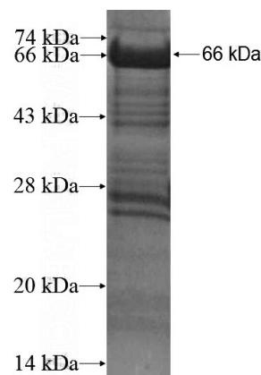
Recombinant Human RFFL SDS-PAGE
