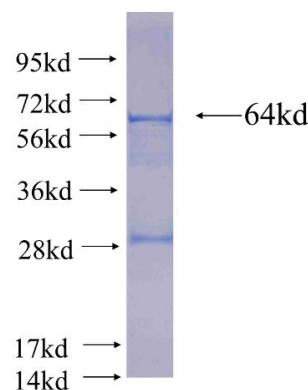
Recombinant human MTHFD2(Full length) SDS-PAGE
