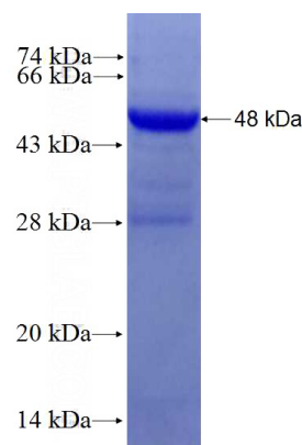
Recombinant Human COQ3 SDS-PAGE
