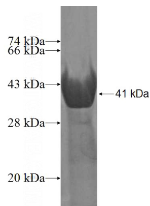
Recombinant Human NAB2 SDS-PAGE
