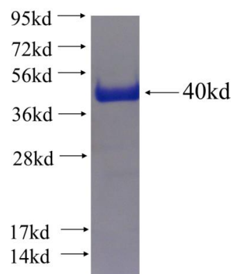
Recombinant human ZFYVE28 SDS-PAGE
