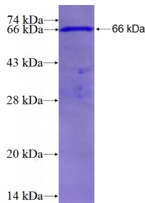
Recombinant Human SEPT1 SDS-PAGE
