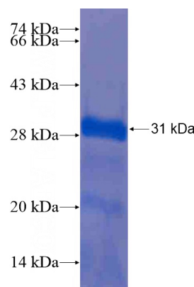
Recombinant Human IL-27 SDS-PAGE
