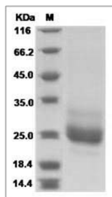
GPIHBP1 protein SDS-PAGE
