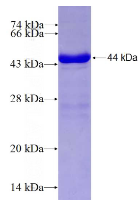
Recombinant Human CLPTM1 SDS-PAGE
