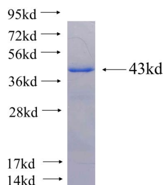
Recombinant human PGRMC1 SDS-PAGE
