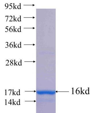
Recombinant human RAB7B SDS-PAGE
