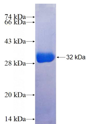
Recombinant Human PRUNE2 SDS-PAGE
