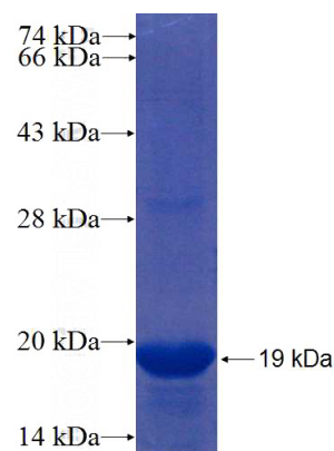
Recombinant Human ZNF193 SDS-PAGE
