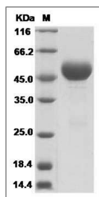
Mouse Alpha 1 Antitrypsin / SerpinA1a Protein (His Tag) SDS-PAGE
