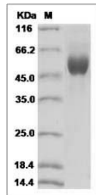
HA protein SDS-PAGE
