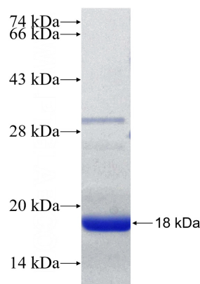
Recombinant Human SETD3 SDS-PAGE
