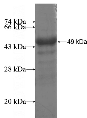
Recombinant Human RNF133 SDS-PAGE
