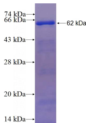
Recombinant Arabidopsis thaliana SHM7 SDS-PAGE
