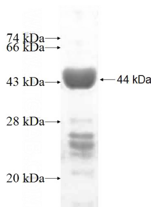
Recombinant Human PABPC4 SDS-PAGE
