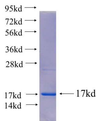
Recombinant human TTC39A SDS-PAGE
