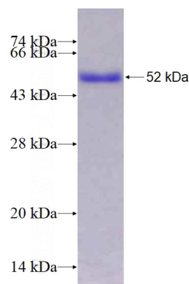
Recombinant Human SMAD7 SDS-PAGE
