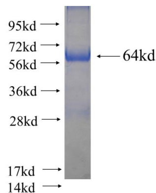
Recombinant human UNR; CSDE1 SDS-PAGE
