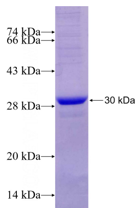
Recombinant Human POLQ SDS-PAGE
