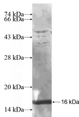
Recombinant Human UCP1 SDS-PAGE
