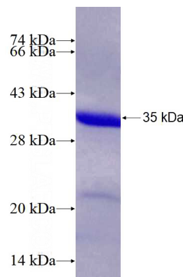
Recombinant Human HFM1 SDS-PAGE
