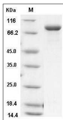
Mouse Transferrin Receptor / TFRC / CD71 Protein (His Tag) SDS-PAGE
