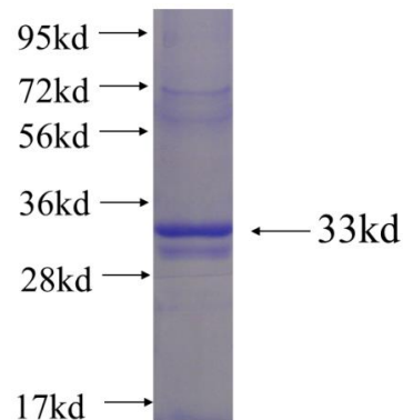
Recombinant human PTCD2 SDS-PAGE
