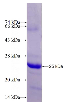
Recombinant Human DNAJB9 SDS-PAGE
