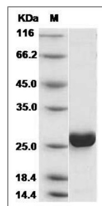
Human CMPK1 Protein (His Tag) SDS-PAGE
