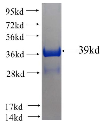
Recombinant human PSMG3 SDS-PAGE
