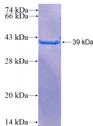
Recombinant Human RBL2 SDS-PAGE
