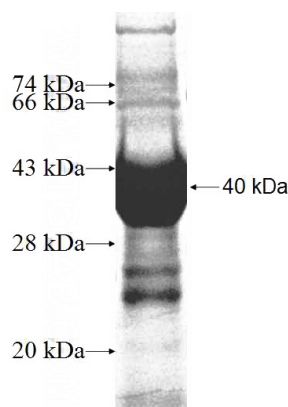
Recombinant Human NFKBIL2 SDS-PAGE
