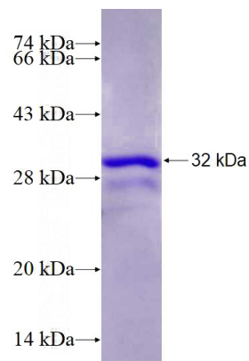
Recombinant Human USPL1 SDS-PAGE
