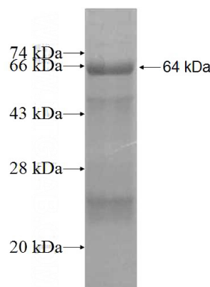
Recombinant Human LSS SDS-PAGE
