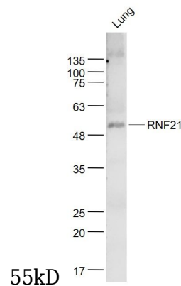
Fig2: Sample:; Lung (Mouse) Lysate at 40 ug; Primary: Anti- RNF21 at 1/1000 dilution; Secondary: IRDye800CW Goat Anti-Rabbit IgG at 1/20000 dilution; Predicted band size: 57kD; Observed band size: 55 kD
