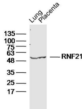
Fig1: Sample:; Lung (Mouse) Lysate at 40 ug; Placenta (Mouse) Lysate at 40 ug; Primary: Anti-RNF21 at 1/300 dilution; Secondary: IRDye800CW Goat Anti-Rabbit IgG at 1/20000 dilution; Predicted band size: 57kD; Observed band size:
