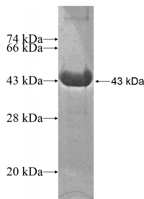
Recombinant Human USH1G SDS-PAGE
