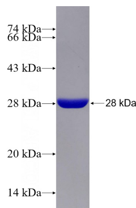
Recombinant Human SF3B4 SDS-PAGE
